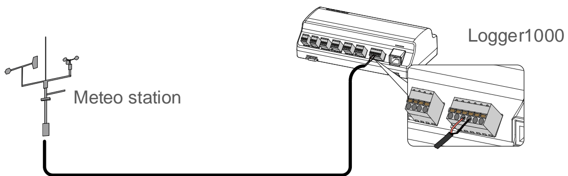
Figure 2-1 RS485 Connection
