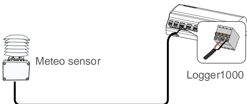
Figure 2-2 AI Connection
